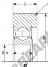
Bearing Flush with Inner Edge Style 1: Standard Conrad style with radius
