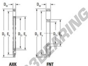
Boundary dimensions
