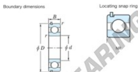
Deep groove Ball Bearing - Single Row - Locating snap ring
