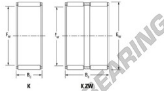
Roller and cage assemblies
