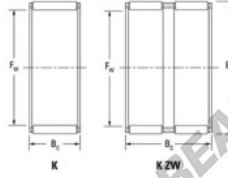
Boundary dimensions
