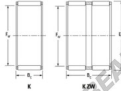
ISO 3320 Needle roller and cage assemblies
