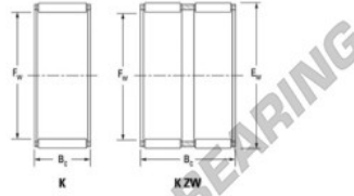
Radial needle roller and cage assemblies
