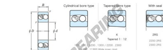
Boundary dimensions
